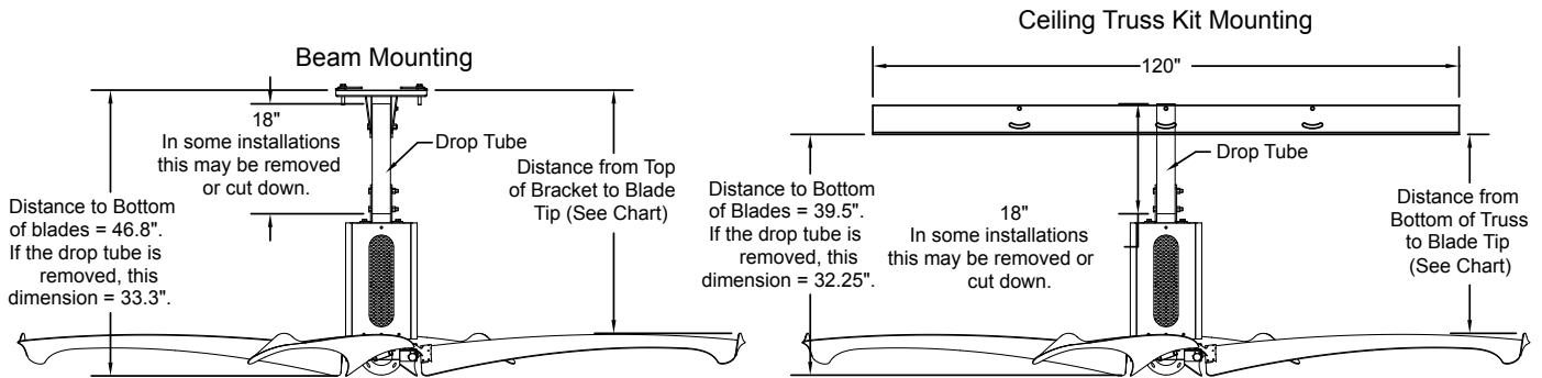
Ceiling Truss Kit Mounting
